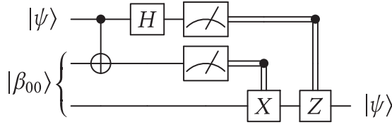
Fig. 4. The quantum teleportation circuit, where |\beta_{00}\rangle = \frac{|00\rangle + |11\rangle}{\sqrt{2}} . The last two quantum gates Z and X are controlled by the measurement result of the top two qubits.
